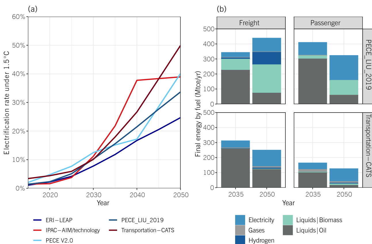
FIGURE 4-19. ELECTRICITY PERCENTAGE IN TOTAL TRANSPORTATION ENERGY CONSUMPTION (PANEL A) AND TWO ILLUSTRATIVE SCENARIOS OF ENERGY DEMAND AND FUEL MIX IN THE TRANSPORTATION SECTOR (PANEL B).
