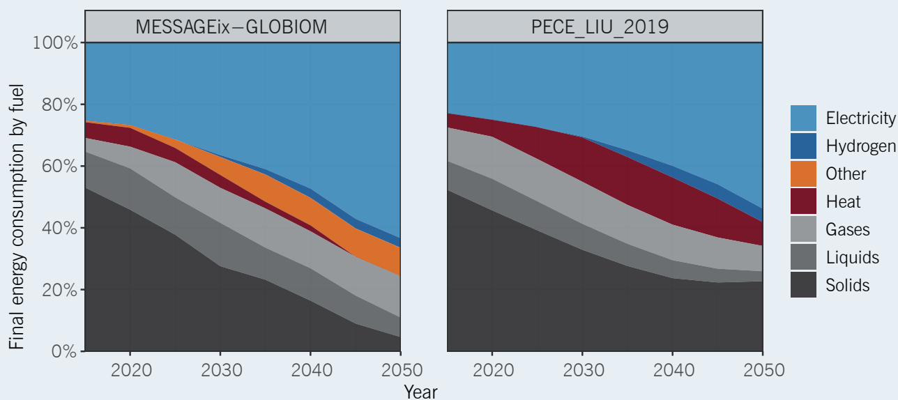
FIGURE 2. INDUSTRIAL FINAL ENERGY STRUCTURE FROM TWO ILLUSTRATIVE 1.5°C SCENARIOS.
