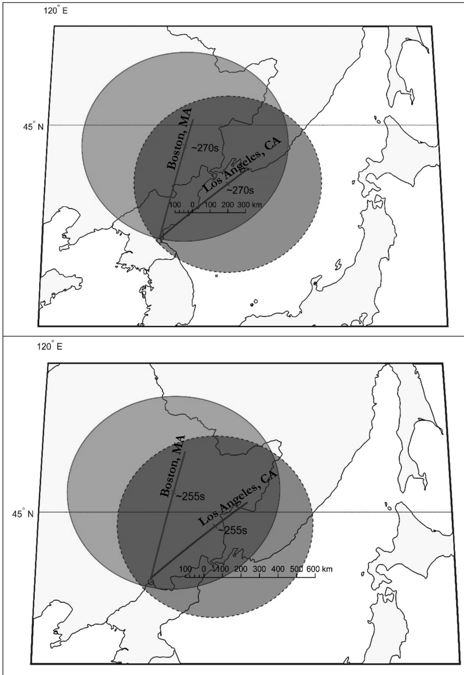
Figure 2. Interceptor Basing Area Plots for North Korean Hwasong-15 ICBM
